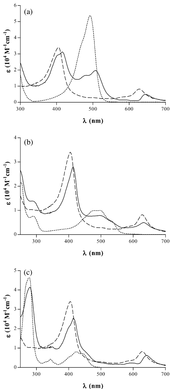
Fig. 4. Absorption spectra of CHL (dashed line), each of the mutagens studied alone (dotted lines) and computed spectra of (a) AO-CHL, (b) Dox-CHL and (c) QM-CHL (solid lines).
